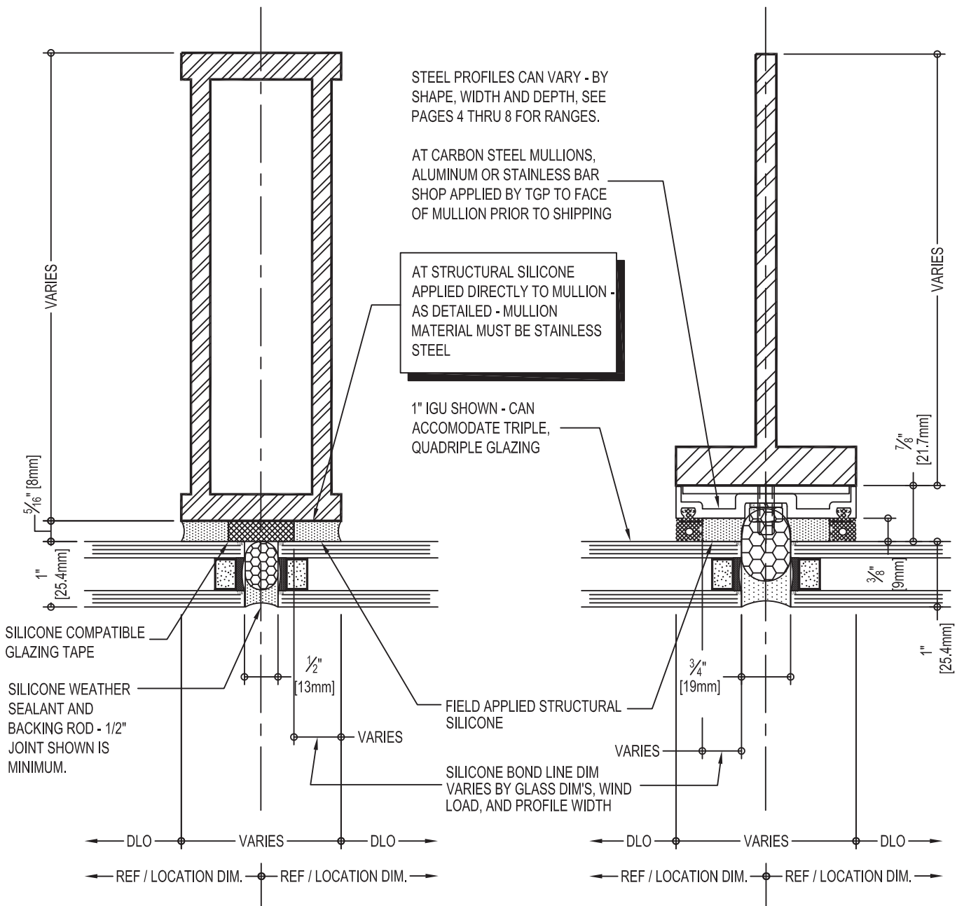
STRUCTURAL SILICONE GLAZING / MULLION
